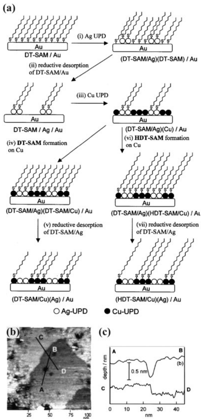
Figure 5.20 (a) Scheme of generation of mixed SAMs and nanopores using UPD of Ag and Cu. (b) STM image of a sample prepared by the sequence of steps i–v. (c) height profiles with lines A–B and C–D crossing a nanopore and a substrate step. Reproduced with permission from Ref. [220].
