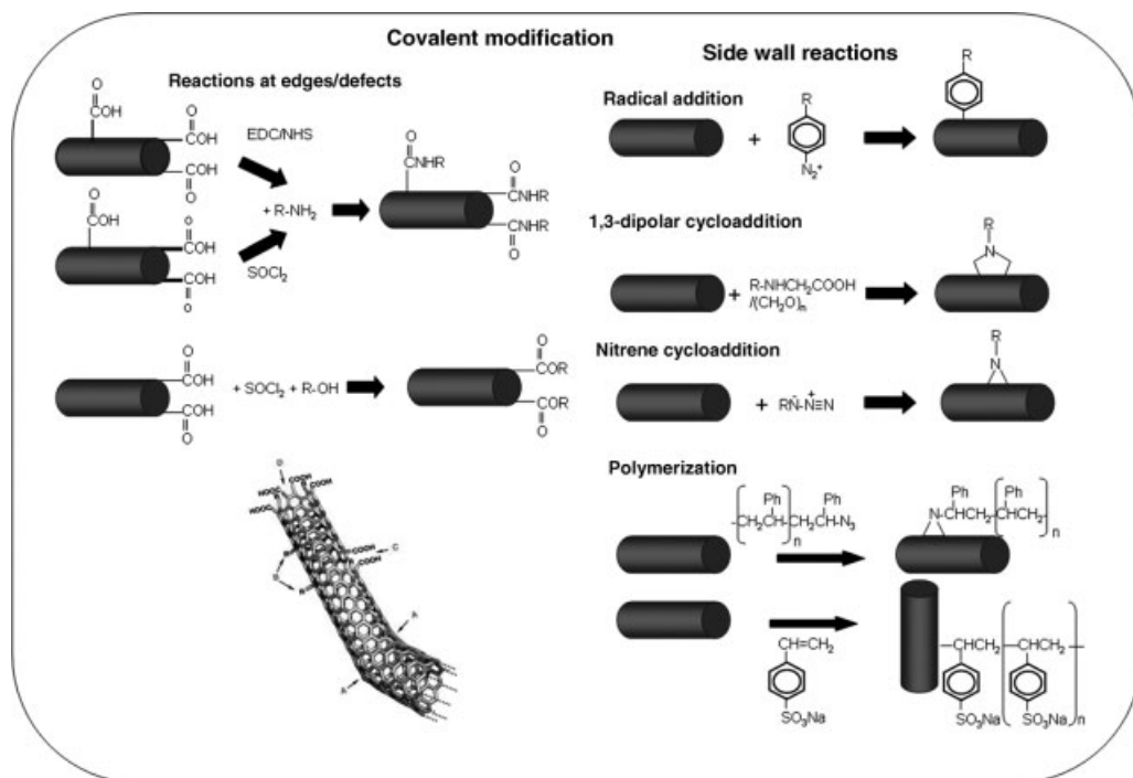
Figure 3.8 Scheme showing the more common covalent reactions at the CNT edge/defects and at the CNT sidewalls. The figure also shows the typical defects in a SWNT: (a) five- or seven-membered rings in the C network, instead of the normal six-membered ring, leads to a bend in the tube, (b) sp^3 -hybridized defects
