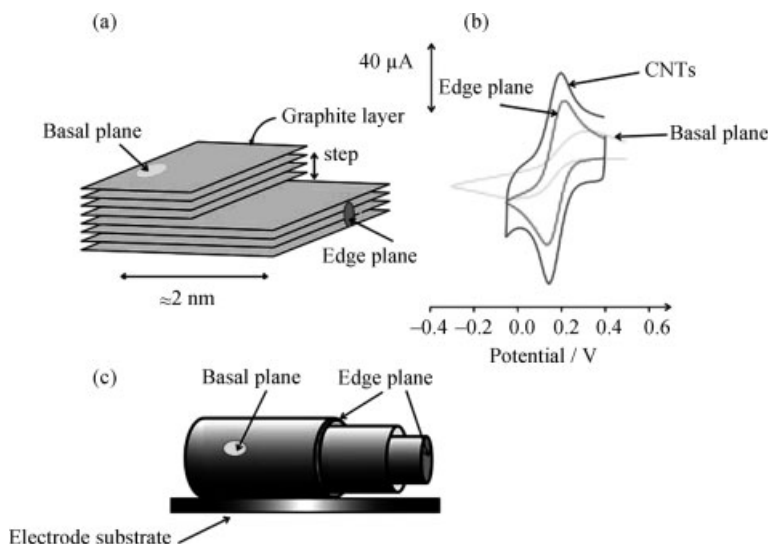
Figure 3.6 (a) Schematic representation of the layered structure of HOPG with the indication of the different edge and basal planes. (b) Voltammetric response of \text{Fe}(\text{CN})_6^{3-/4-} using basal-plane, edge-plane pyrolytic graphite and CNT electrodes. (c) Scheme of a MWNT on an electrode surface showing the edge plane and basal plane like sites. Reprinted with permission from Ref. [64]. Copyright, 2006, Wiley-VCH Verlag.
