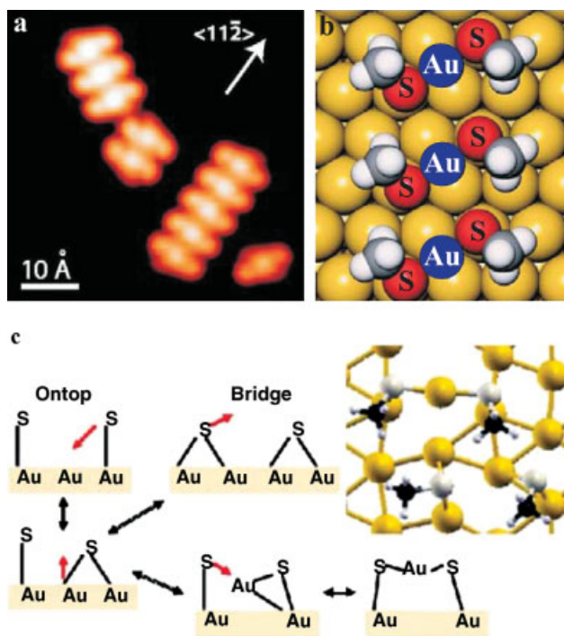
Figure 5.4 STM image and models of \text{CH}_3\text{S} on \text{Au}(111) . (a) STM micrograph of stacks of \text{CH}_3\text{S-Au-SCH}_3 on \text{Au}(111) recorded at T = 5\text{ K} . Structure was obtained by dissociating adsorbed \text{CH}_3\text{SSCH}_3 at 300\text{ K} . (b) Model of proposed structure with gold adatoms labelled as Au. (c) Structures of \text{CH}_3\text{S} obtained by MD
