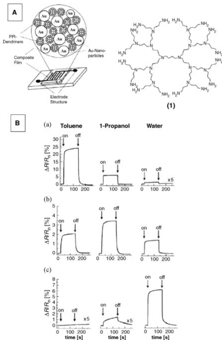
Figure 1.3 (A) Chemresistor containing gold nanoparticles and PPI. (Reprinted with permission ©2002 American Chemical Society.) (B) Response of the Au nanoparticle film to toluene, 1-propanol and water: (a) Au/PPI; (b) Au/PPI; (c) Au/PAMAM. (Reprinted with permission ©2003 Elsevier.) (Reproduced with permission from Ref. [25] © 2004 Wiley-VCH Verlag GmbH & Co. KGaA.)
