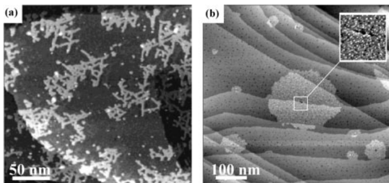
Figure 5.18 In-situ STM images recorded in \text{CuSO}_4/\text{H}_2\text{SO}_4 electrolyte of Cu UPD growth on Au(111) modified by two different types of thiols. (a) SAM of ethane thiol ( 250 \times 250 \text{ nm}^2 ) with a ramified structure and (b) SAM of MBP2 ( 600 \times 600 \text{ nm}^2 ) with circular copper patches [43]. Enlarged area reveals nanometer-sized islands protruding on patches. (a) Reproduced with permission from Ref [210].
