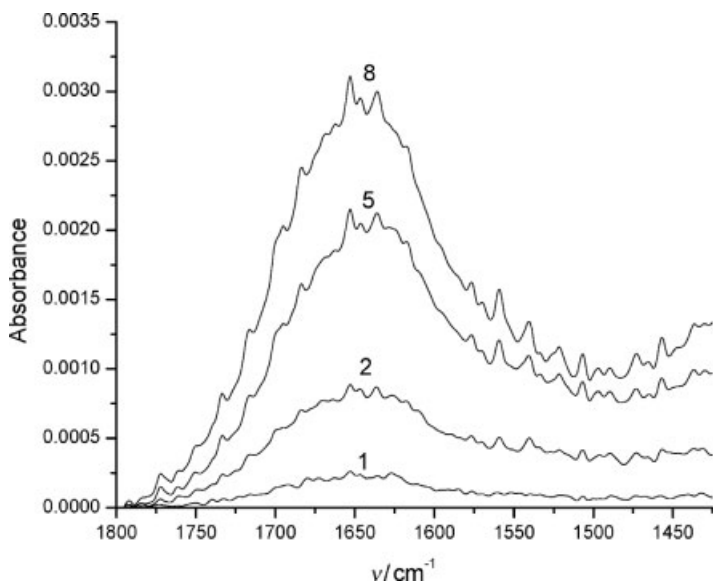
Figure 2.21 FT-IRRAS spectra for the \text{H}_2\text{O} band 1648\text{ cm}^{-1} (PAH-Os(II)) 15 (PSS) 15 . Numbers indicate the oxidation–reduction cycle number. Taken from Ref. [153].
